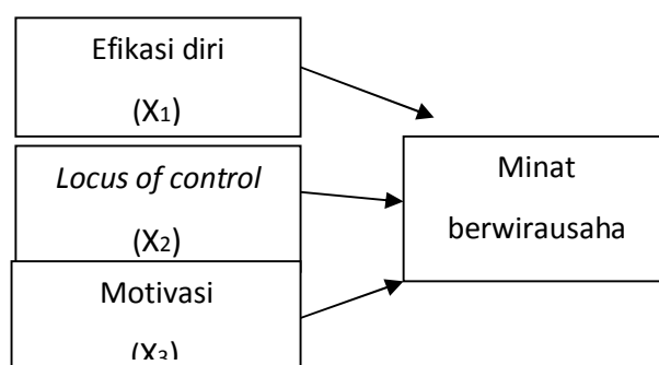
Gambar 2.1 Rerangka penelitian
